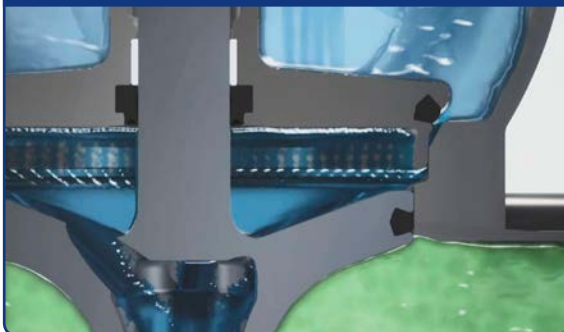
Figure 2. Seat lift: The upper valve plug is raised off the seat thus cleaning plug seal, seat and leakage chamber through CIP flow.
